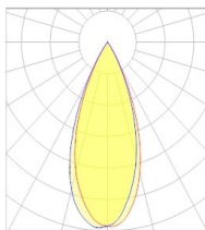
50° Wide beam
