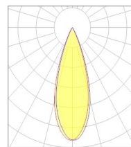
36° Medium beam
